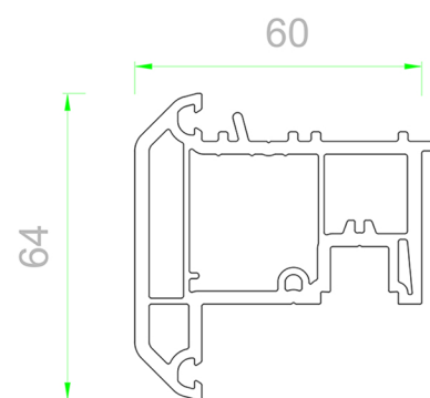
507/05 Overhung
