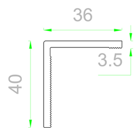
507/22 Renovation Angle 36 mm
