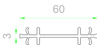
507/13 Coupling
