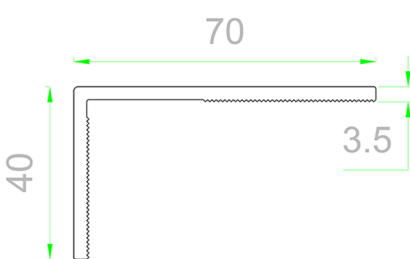
507/12 Renovation Angle 70 mm
