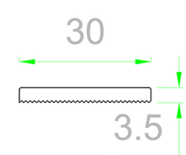
507/25 Strip Profile 30mm
