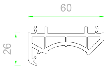
507/10 Bay&Bow adaptor
