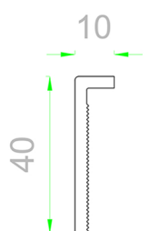
507/23 Renovation Angle 10 mm
