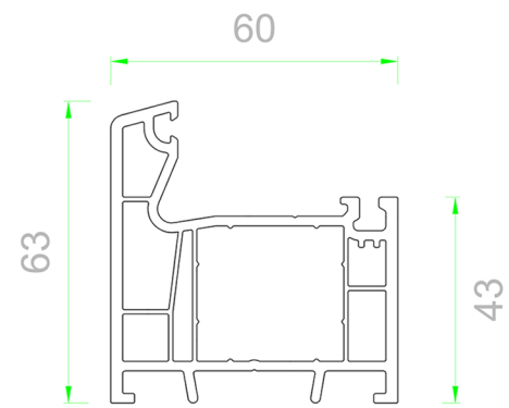
407/01 Frame
