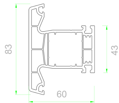
407/03 Mullion
