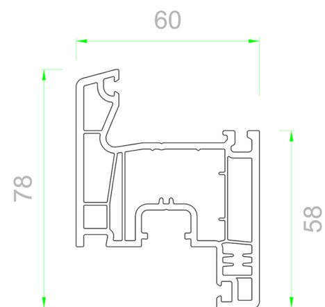
407/16 Sash
