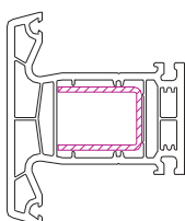
Mullion S-563.03
