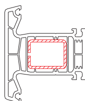
Mullion S-563.03
