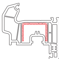
Sash S-563.02
