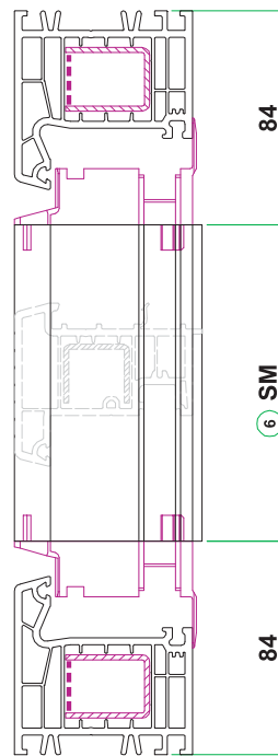
Section C-C
